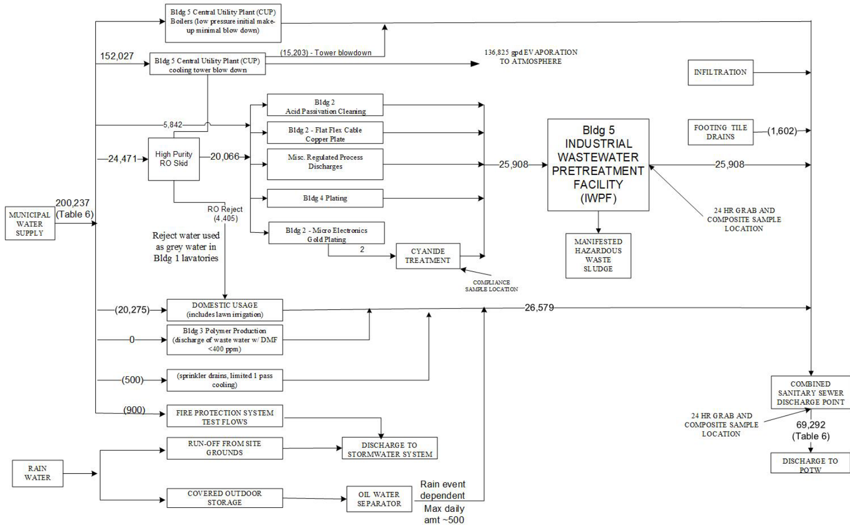
Figure 3-2 Water Balance May 2024 - October 2024
