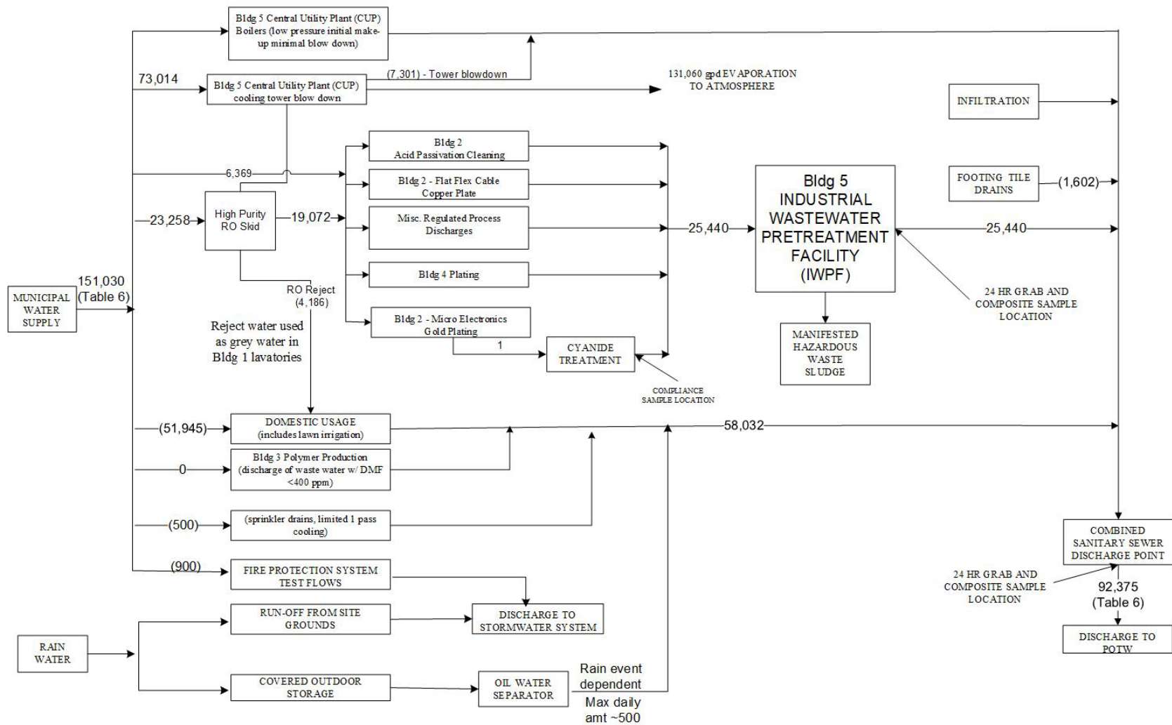
Figure 3-1 Water Balance November 2023 - April 2024
